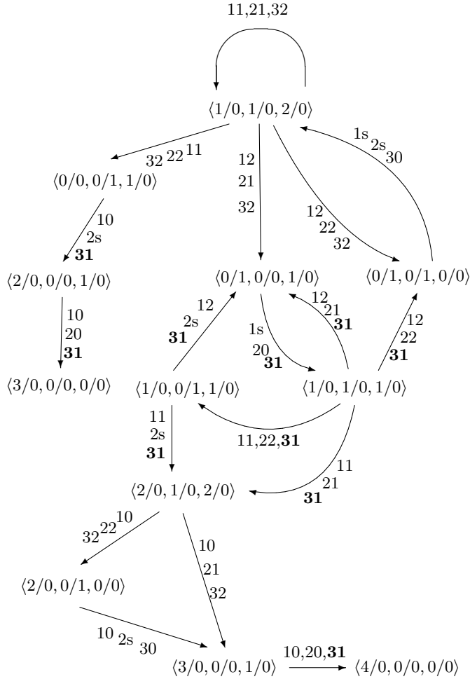
Figure 2: The transition diagram of system II from Figure 1
