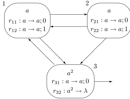
Figure 1: The initial configuration of the SN P system II
