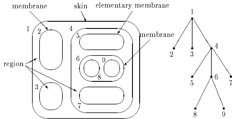
Figure 1: A membrane structure and its associated tree
