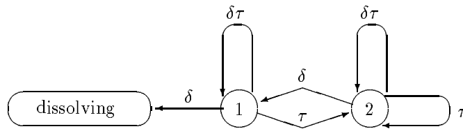
Figure 2: The effect of actions \delta, \tau
